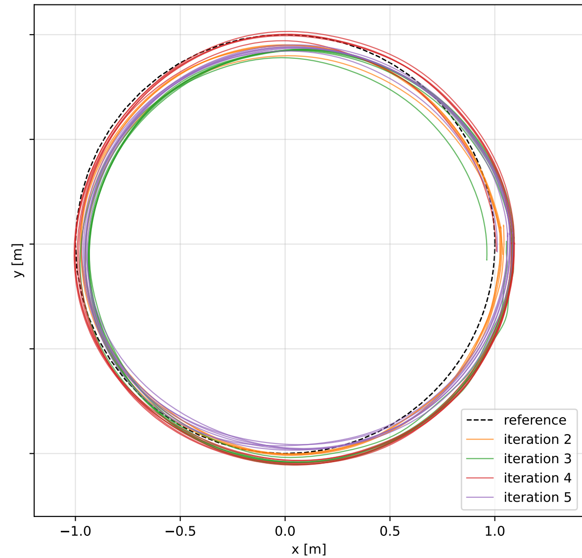
Gain MLP
