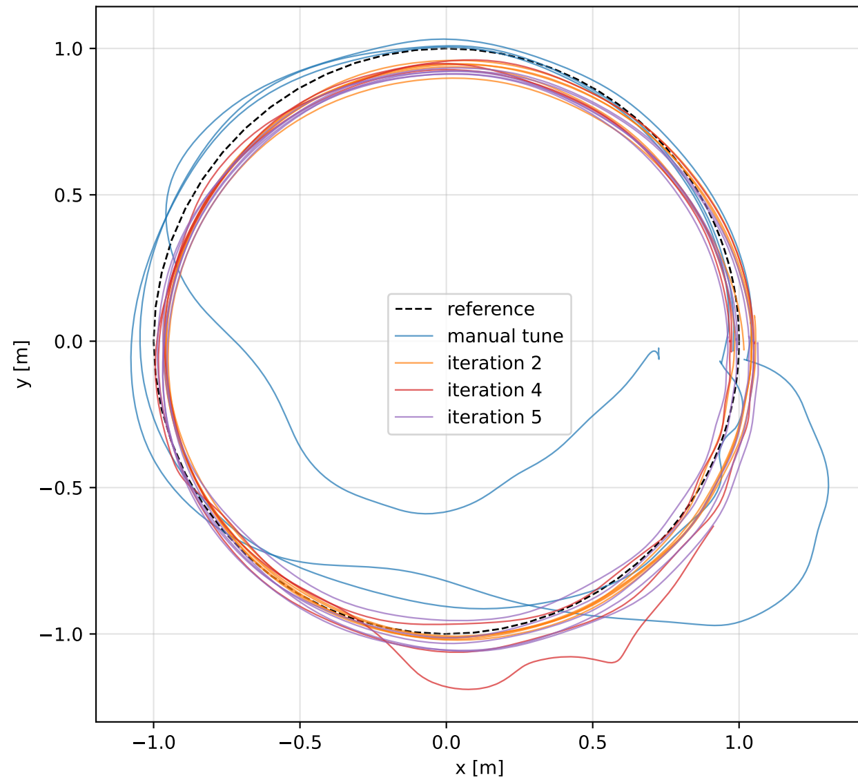
Static Gains
